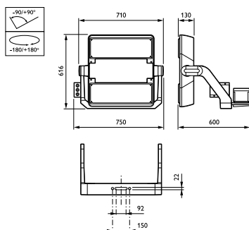
OptiVision LED BVP500-522
